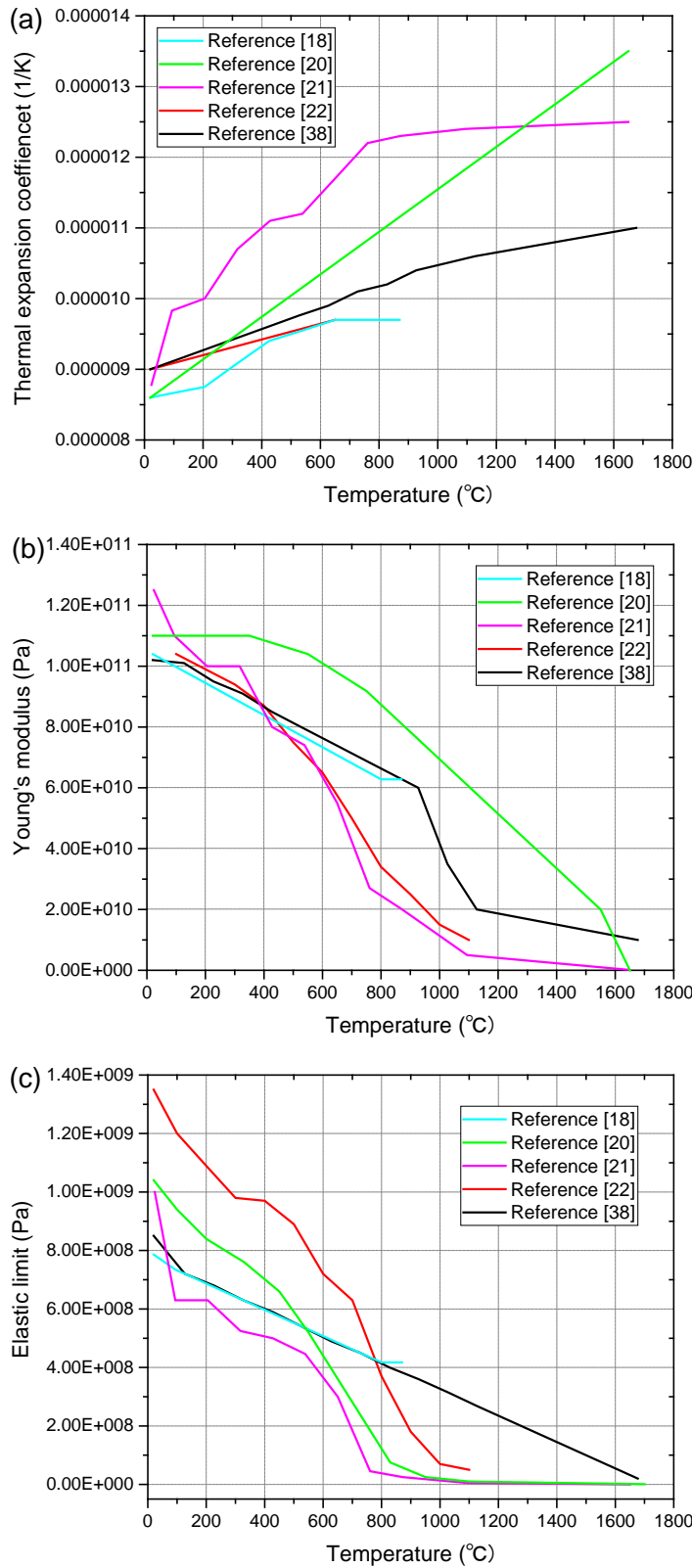
Fig.2 Ti-6Al-4V titanium alloy: mechanical properties.
