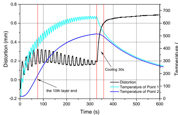
Fig. 11 The evolution of the distortion at the DS position and the calculated temperature evolution at point 1 and point 2, respectively (see Fig.
