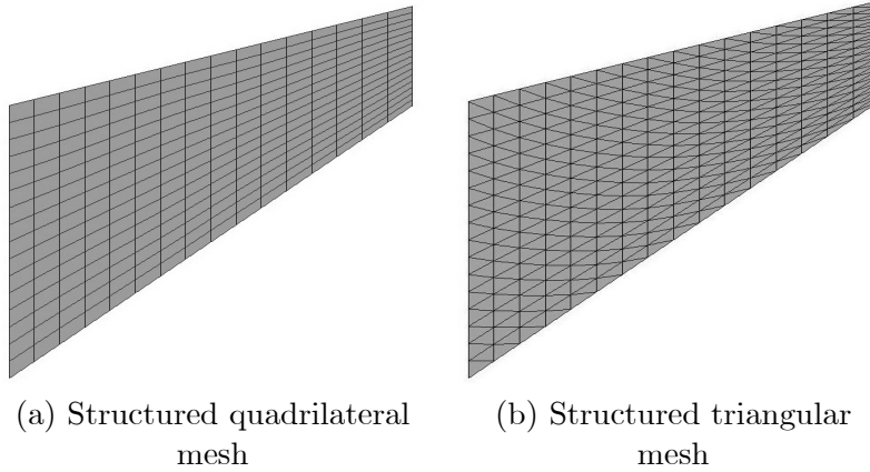
Figure 2: Cook's membrane problem: (16 x 16) FE meshes.
