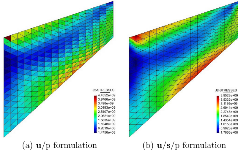
Figure 4: Cook's membrane problem (16x16 triangular mesh): J2 deviatoric stress value.
