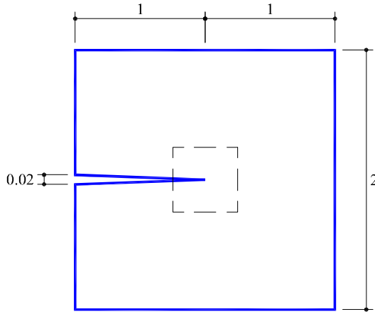
Figure 9: Geometry for the sharp V-notched specimen under tension
