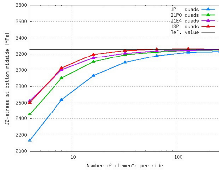
(c) QUAD: J2-stress
