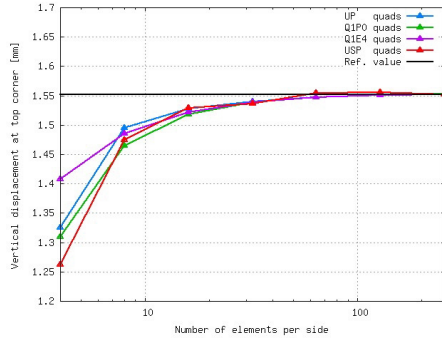
(a) QUAD: displacement
