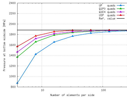
(e) QUAD: pressure
