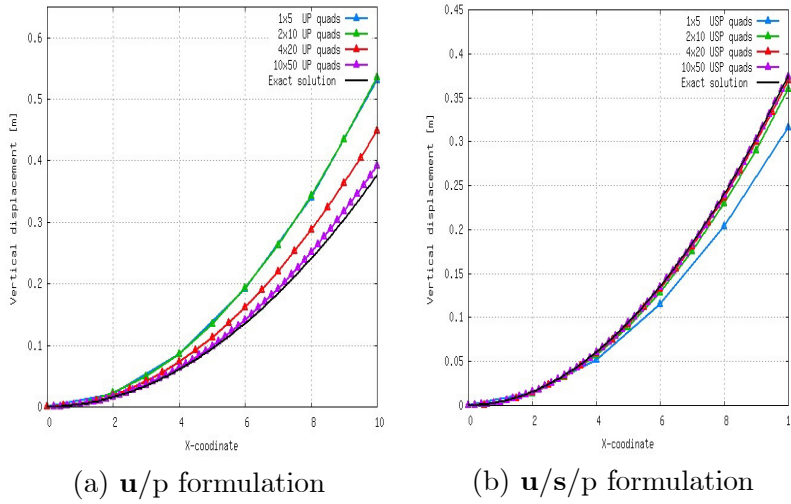
Figure 8: Cantilever beam problem: vertical displacement along the top side of the beam using different mesh resolutions.
