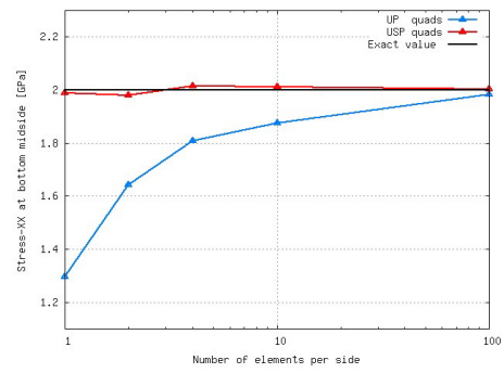
(b) Max. hor. normal stress
