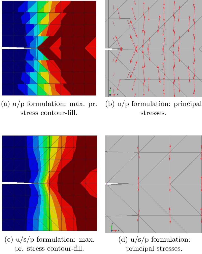
Figure 10: Sharp V-notch specimen under tension. Principal stresses.
