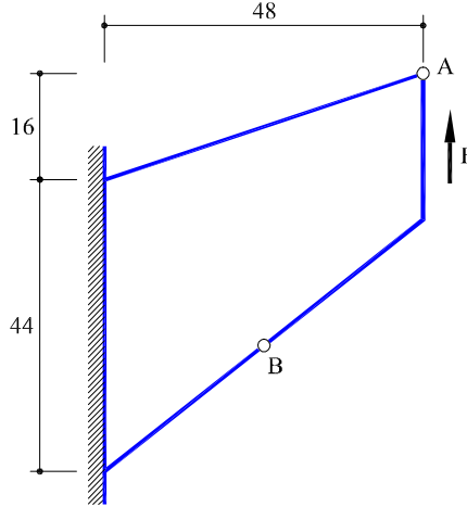
Figure 1: Cook's membrane problem: geometry.
