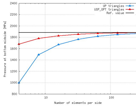
(f) TRI: pressure
