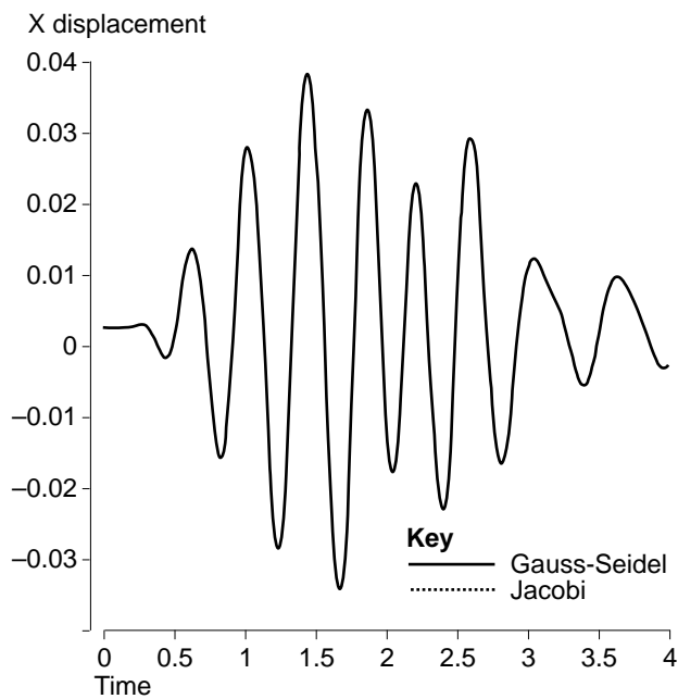
Note: Top horizontal displacement (tolerance = 0.01 per cent)
