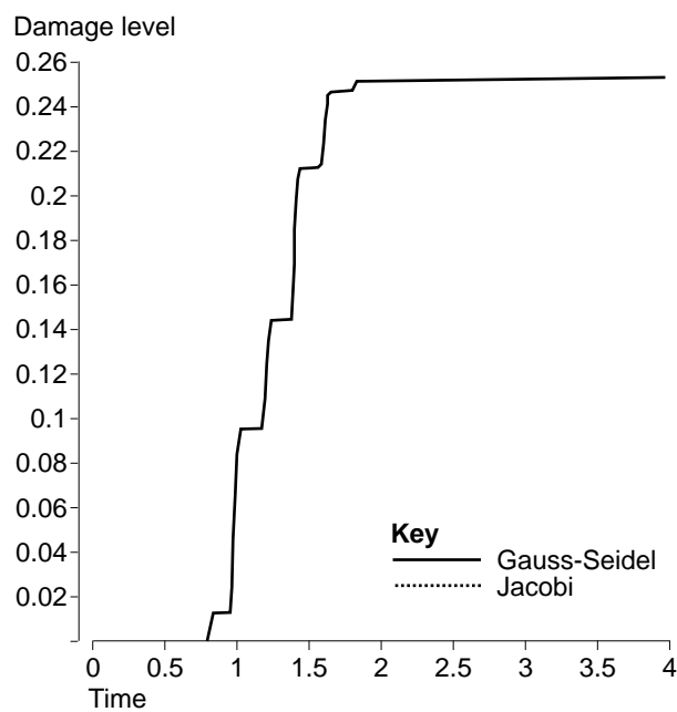
Note: Damage level (tolerance = 0.01 per cent)
